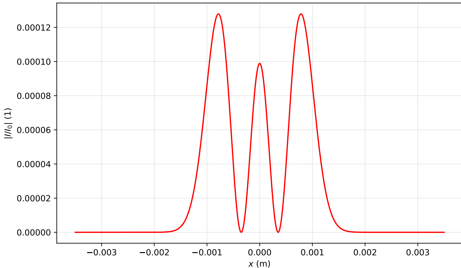
Intensity profile I(x, y = 0, z = 0.080)/I_0 , P_{in}=5.0P_{cr} , artificial time
